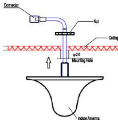
Installation Sketch
