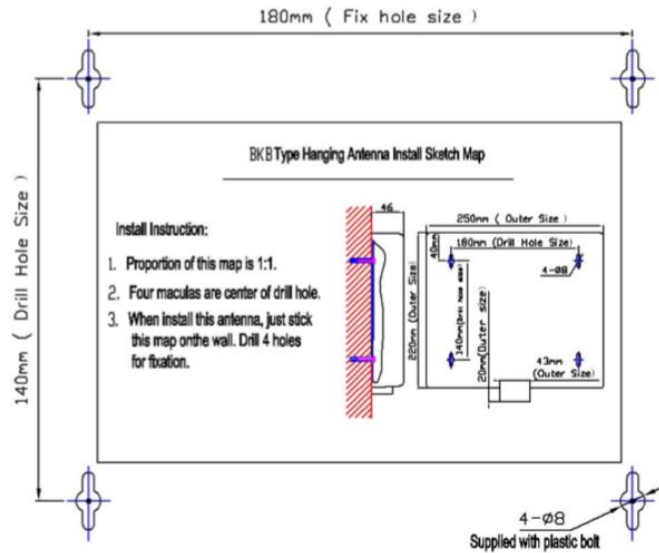
Installation Sketch
